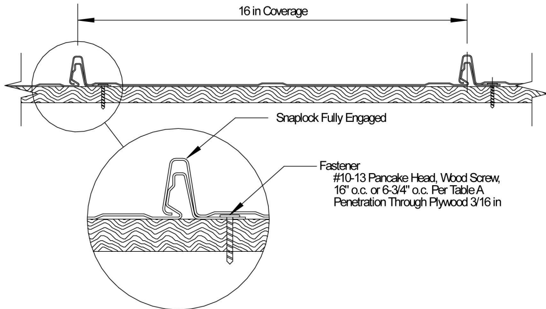
Typical Panel Assembly View (Method 1 & 2 )
